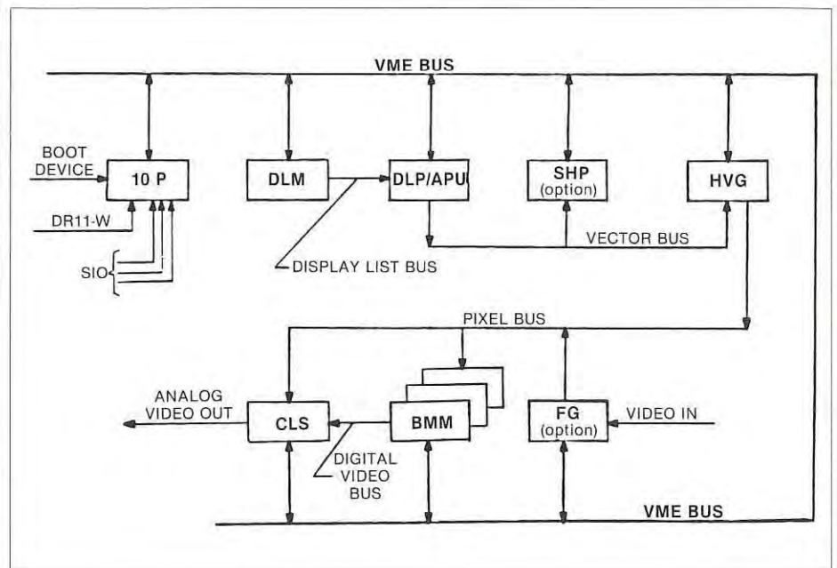
Fig. 3: Block diagram of the graphics engine of Le Mans Colorgraphic by Chromatics, Inc.
