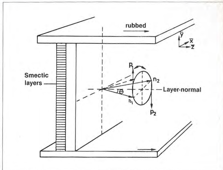
Fig. 3: SSFLC switching.
