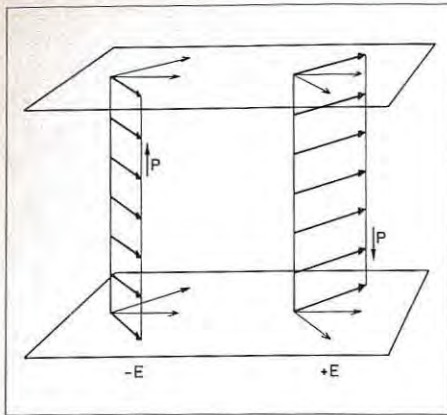
Fig. 2: SSFLC structure.
