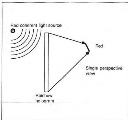
Fig. 5a: Rainbow hologram, monochromatic source.
