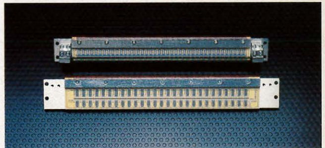
GaAsP LED arrays improve registration by focusing each element at a specific location. Integrally mounted shift register/driver ICs (nitrogen sealed) reduce size and enhance reliability. Wavelength: 660nm. Light output: 4.5uW/st @ 5mA. Compatible with amorphous silicon, organic and selenium photoconductor technologies.
