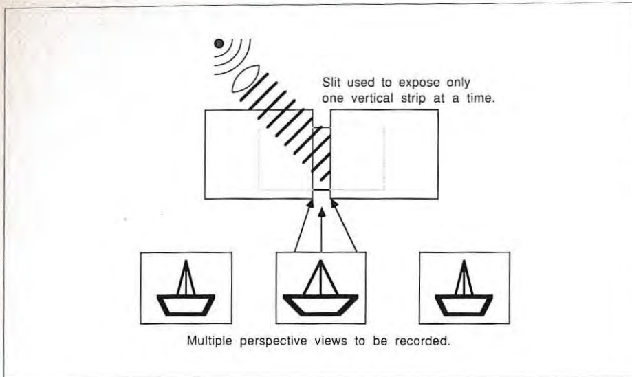
Fig. 4: Recording a holographic stereogram.
