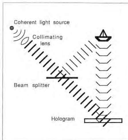
Fig. 2: Recording a transmission hologram.
