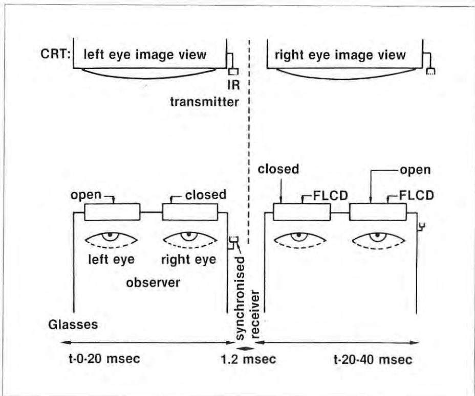
Fig. 1: Field-sequential stereoscopy.
